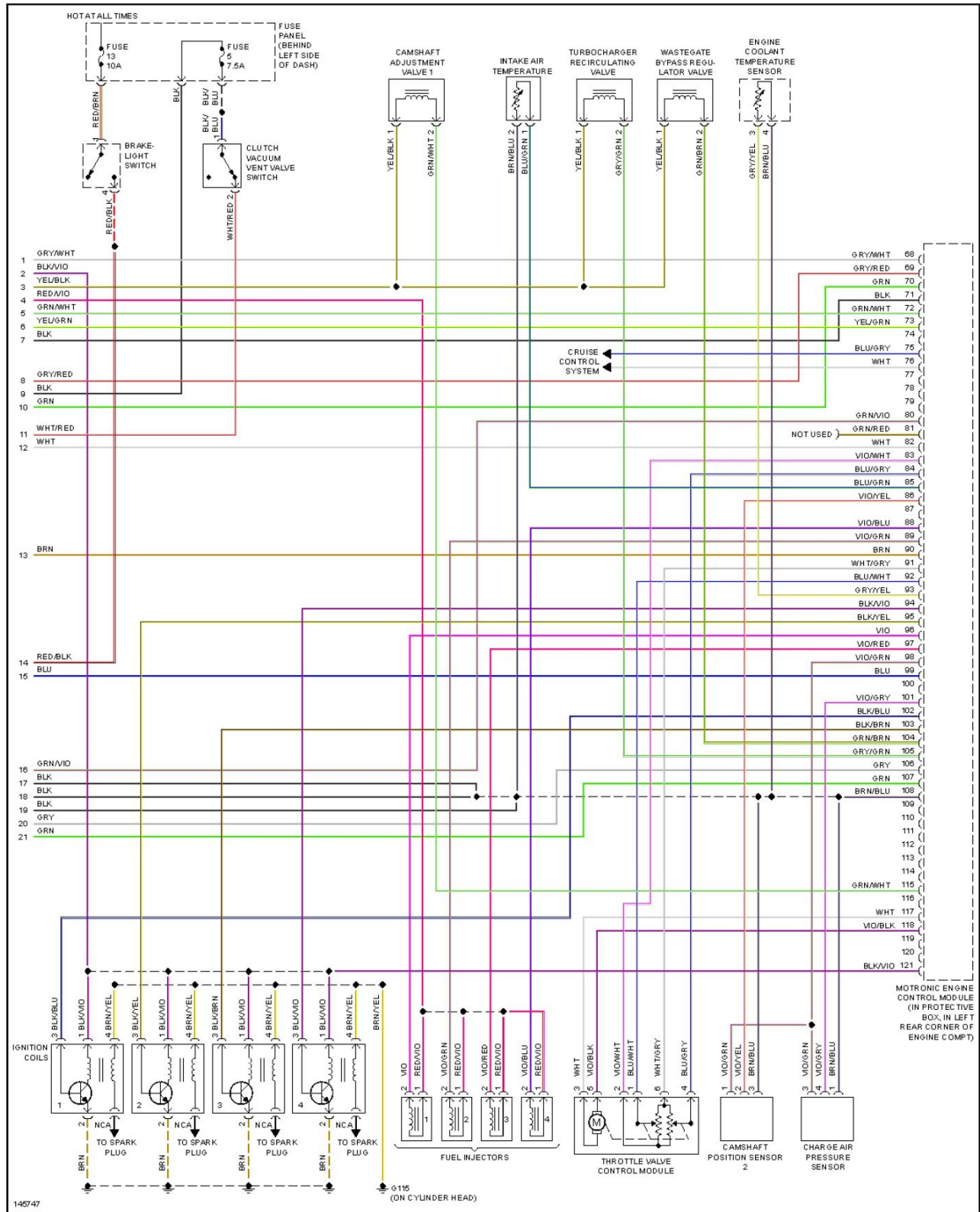
Fig. 28: 1.8L Turbo, Engine Performance Circuits (3 of 3)
