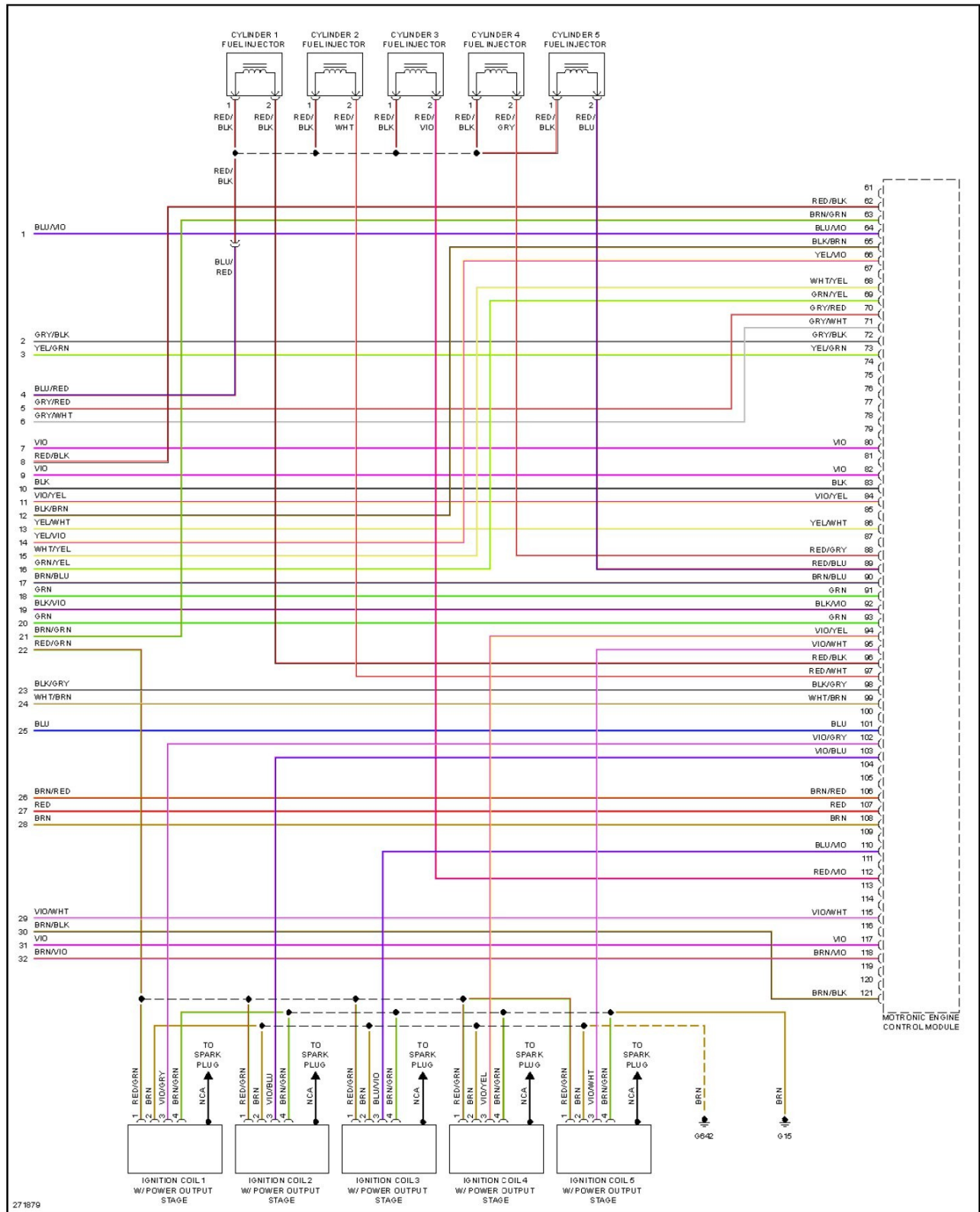
Fig. 36: 2.5L, Engine Performance Circuit, Engine Code BGQ (5 of 5)
