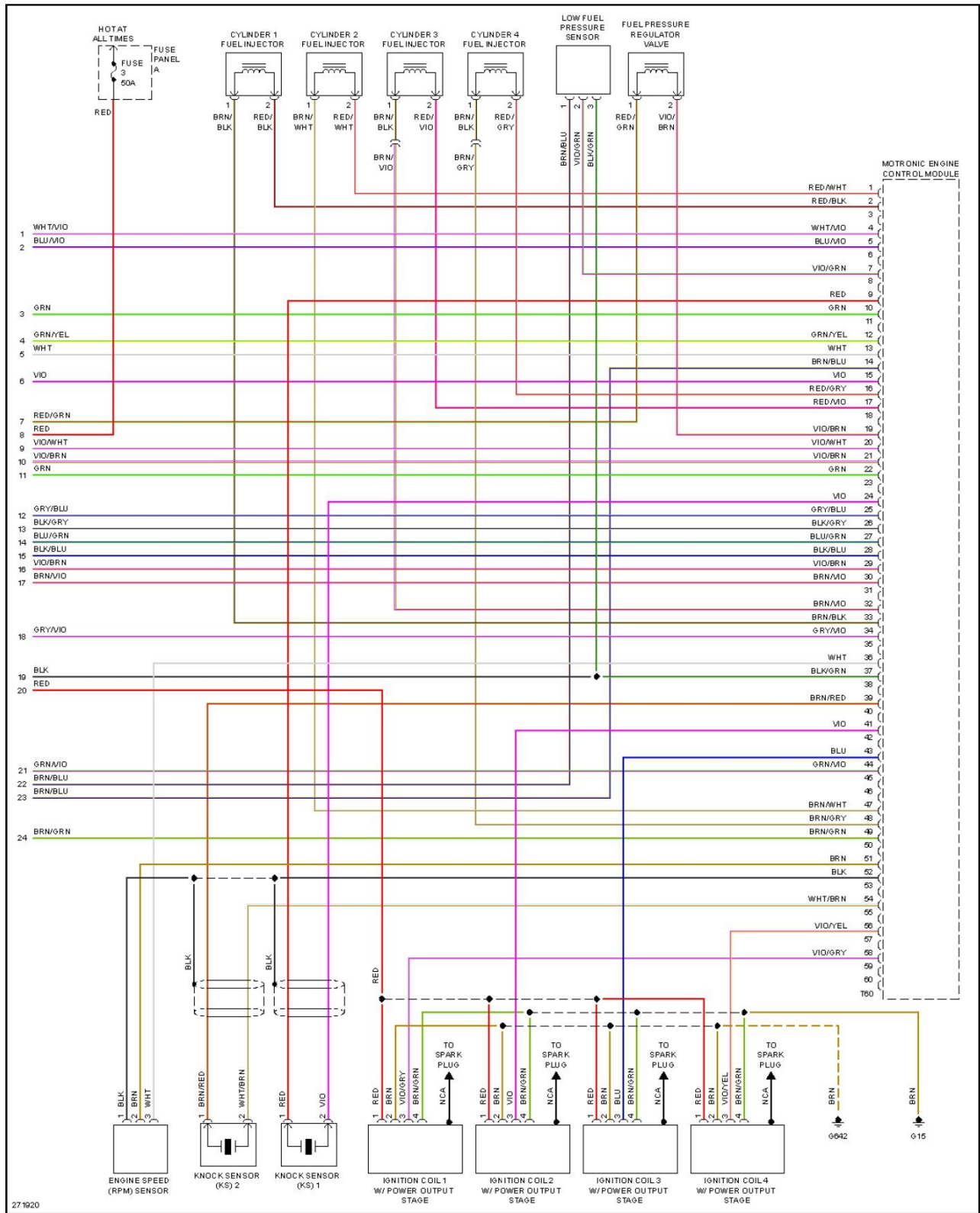
Fig. 26: 2.0L, Engine Performance Circuit (5 of 5)
