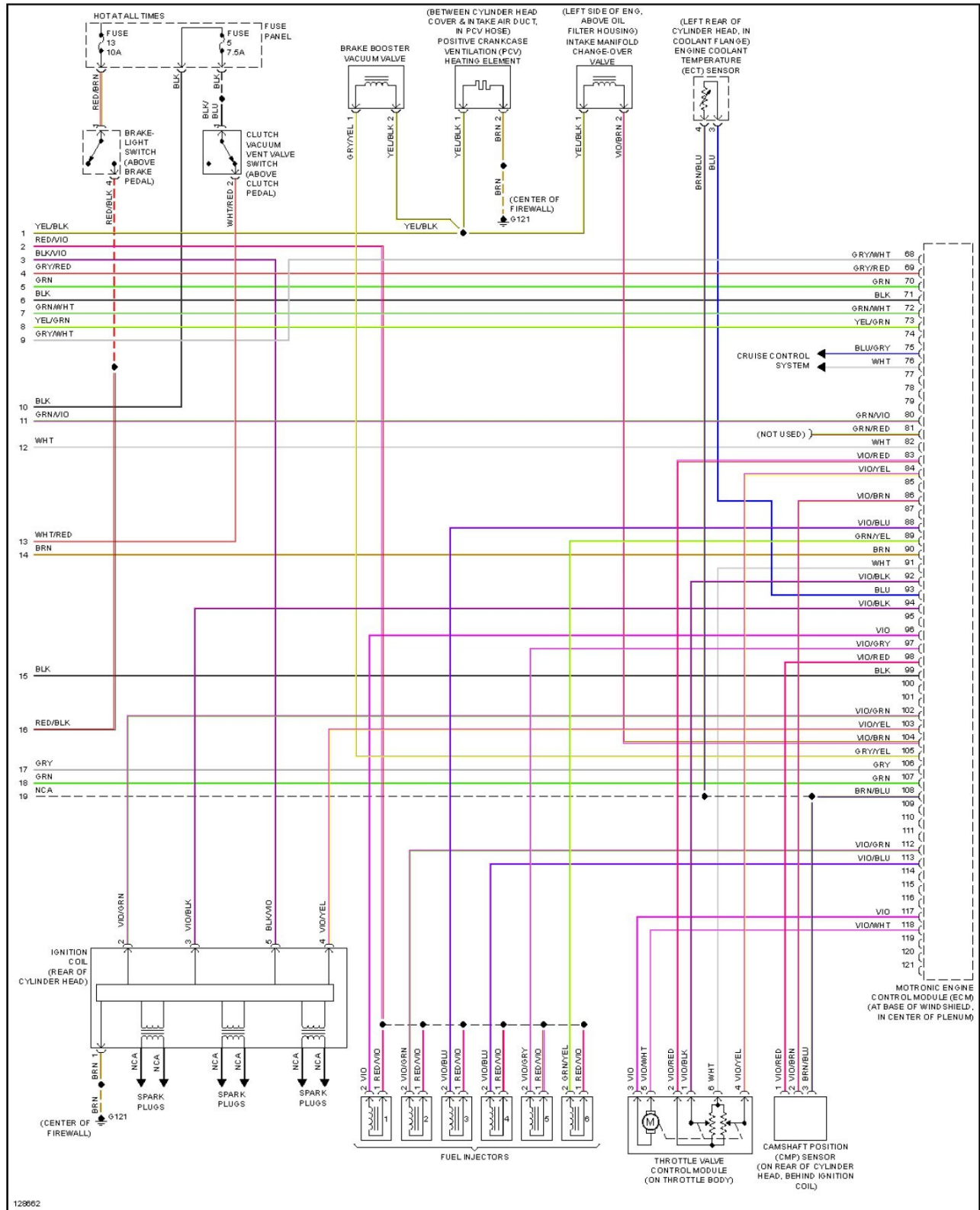
Fig. 40: 2.8L, Engine Performance Circuits (3 of 3)
